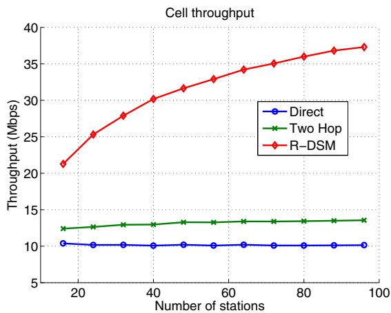
Fig. 6. Cell capacity comparison
